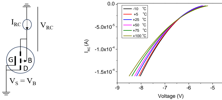
Figure 2: Reader Circuit (RC) configuration and RC-I-V curves at different temperatures
